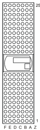
Figure 9-5: Connector X1 (mating side)
