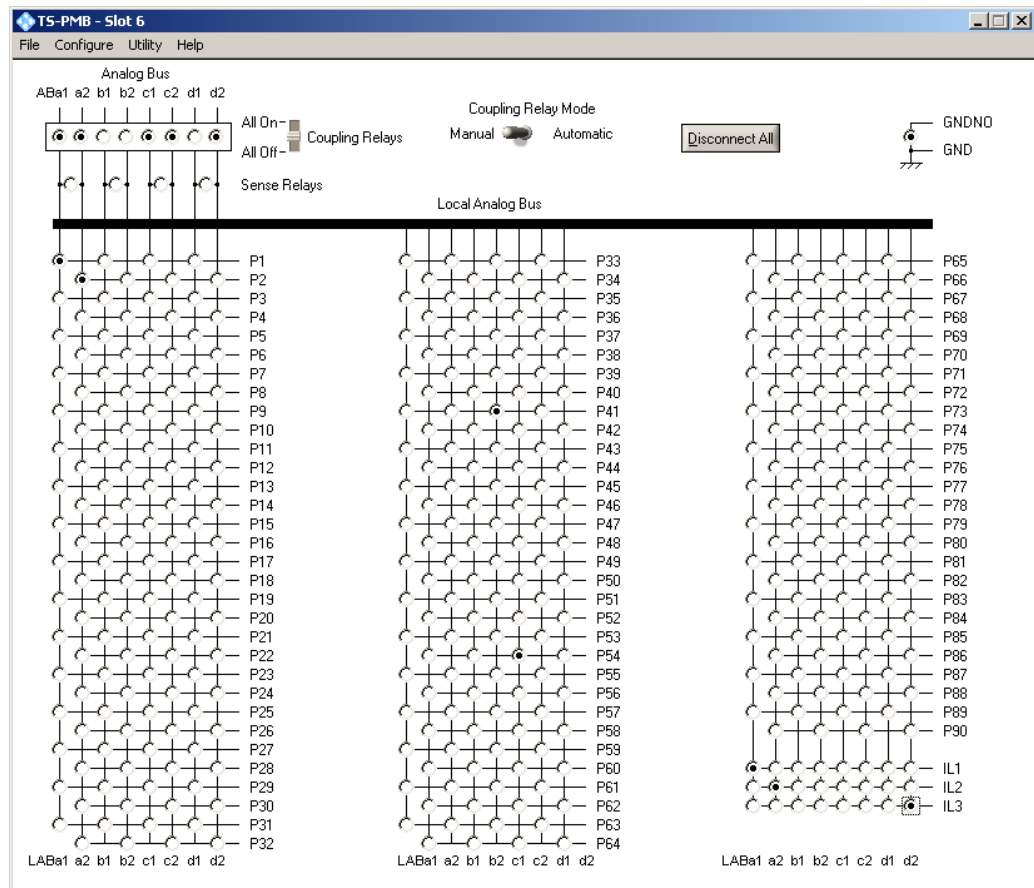
Figure 7-1: Softpanel R&S TS-PMB (example)
