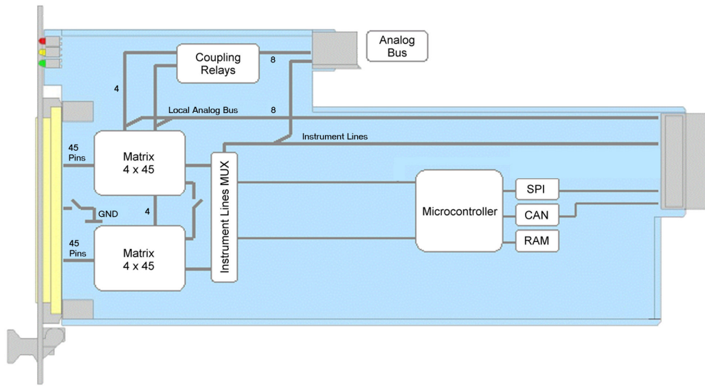
Figure 3-2: Functional Block Diagram R&S TS-PMB
